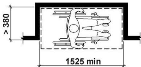
Figure 12: Manoeuvring Clearance in an Alcove, Parallel Approach
